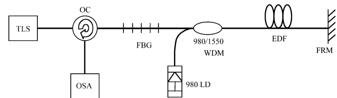
Fig. 1. Schematic diagram of the suggested L -band EDFA.
