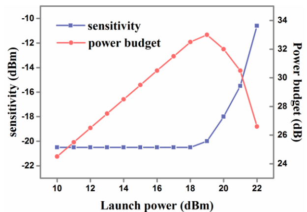
Fig. 8. Required optical power over 40 km SMF for a BER of 10^{-3} versus launch power
