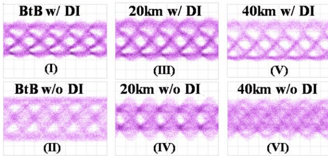
Fig. 6: Insets (I) to (VI) are the eye diagrams of the 25.59-Gb/s downstream signal at back-to-back case and after 20 and 40-km SMF transmission w/ and w/o DI equalization
