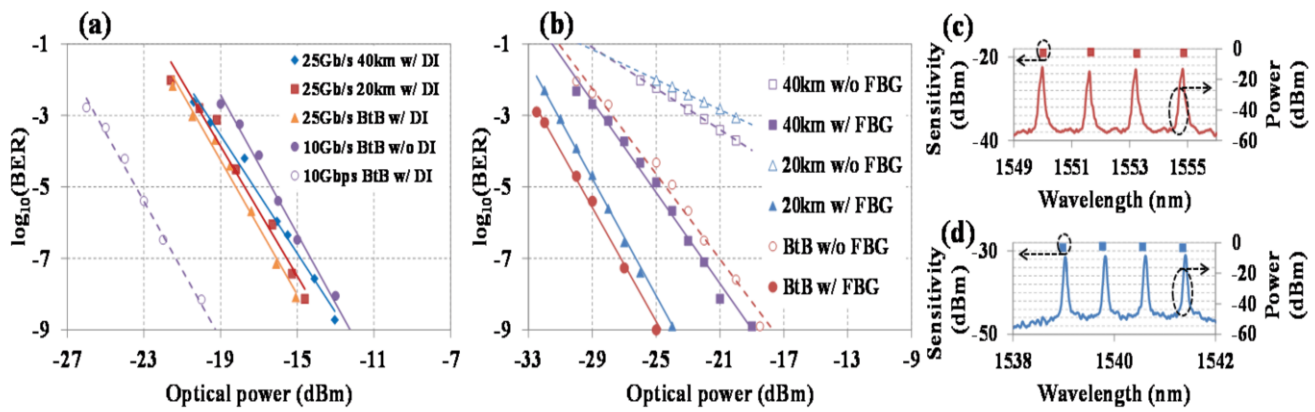
Fig. 9: BER performances versus received optical power for (a) 25.59-Gb/s downstream signal at a wavelength of 1550.1 nm; (b) 10-Gb/s upstream signal at a wavelength of 1539.8 nm. (c) Receiver sensitivity and optical spectra for all the downstream channels; (d) Receiver sensitivity and optical spectra for all the upstream channels
