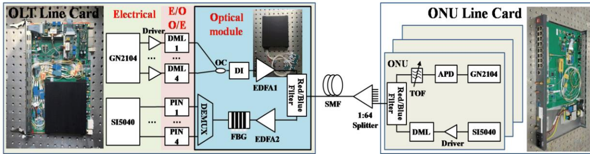
Fig. 1: Transmission scheme of 100G-PON system including the pictures of OLT and ONU line cards
