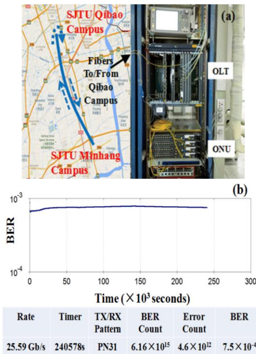
Fig. 10: (a) Map of the round-trip link in SJTU and photo of the 100-Gb/s TWDM-PON systems; (b) BER performance of the downstream signal during 67-h real-time measurement
