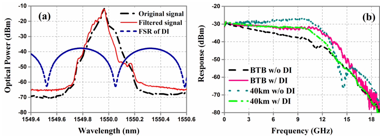
Fig 4: (a) The optical spectra of one downstream wavelength with and without DI and (b) downstream frequency response with and without DI
