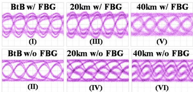
Fig. 7: Insets (I) to (VI) are the eye diagrams of the upstream 10-Gb/s signal at back-to-back case and after 20 and 40 km SMF transmission w/ and w/o FBG compensation
