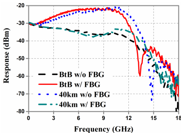
Fig 5: Upstream frequency response with and without FBG
