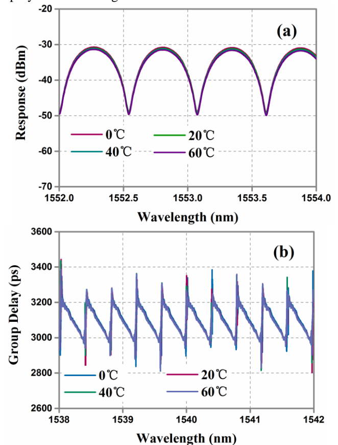
Fig. 3: (a) Spectral response of DI under different temperatures and (b) Group delay profile of FBG under different temperatures
