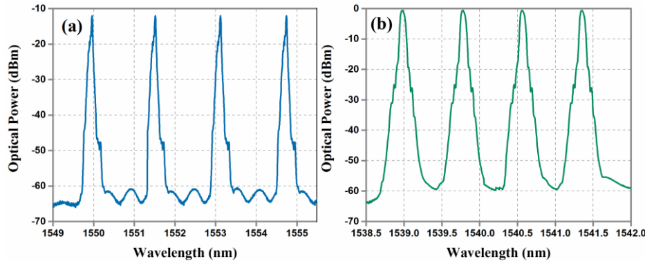
Fig. 2: The measured optical spectra for downstream (a) and upstream (b)
